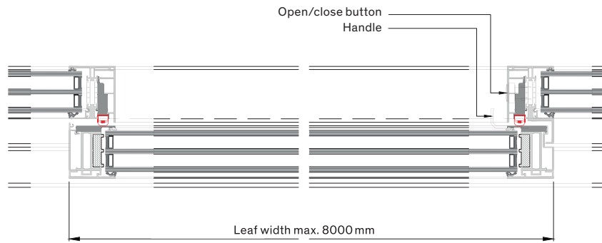
Horizontal cross-section/operation and function
