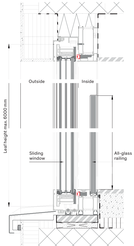
Vertical cross-section/fall protection
