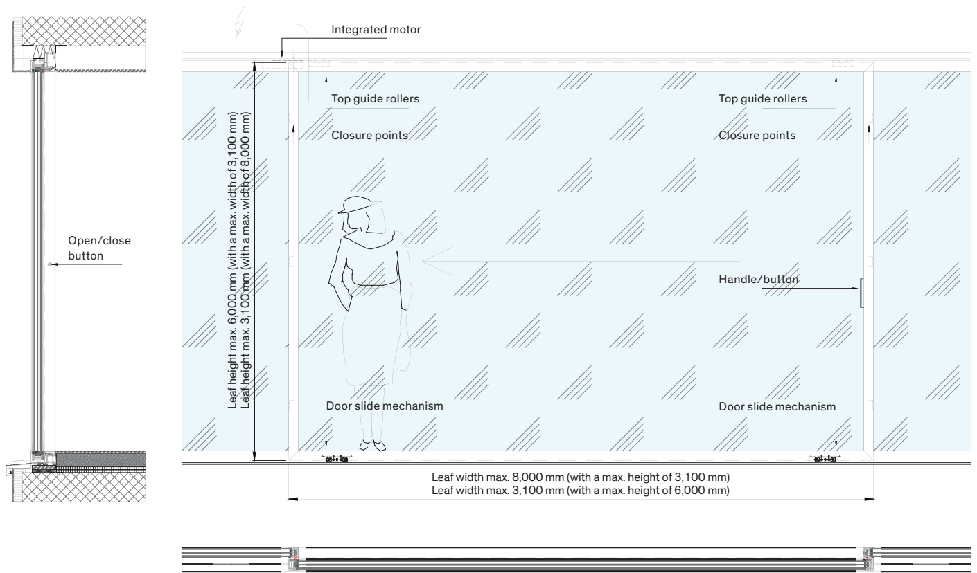
Vertical cross-section/view
