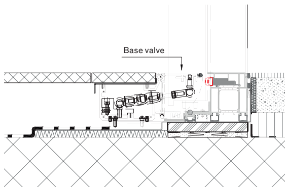
Vertical cross-section/threshold detail
